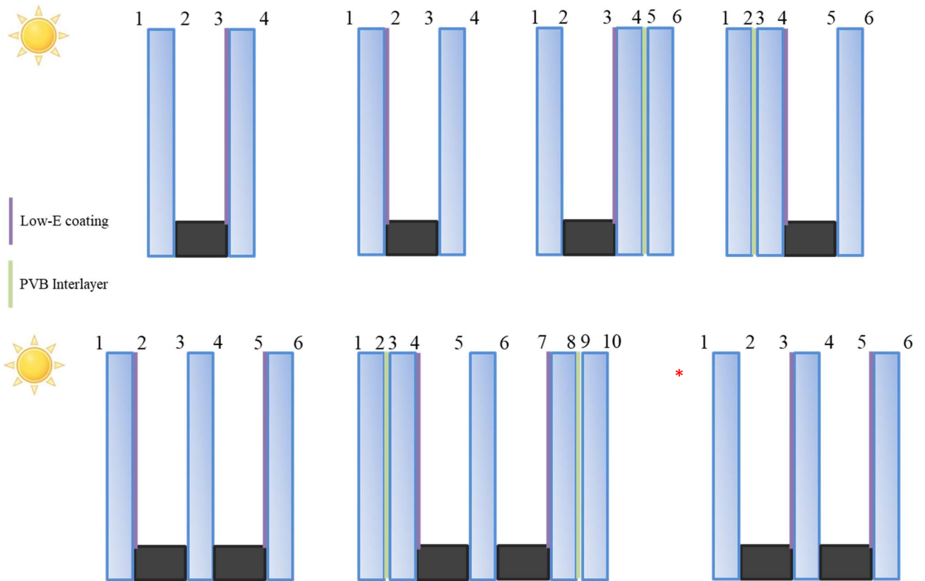
Figure 2: Possible configurations of use of PLANITHERM(II) ® . * Check whether the intermediate coated glass needs to be tempered.
