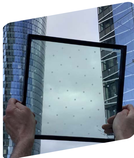
4BIRD®Etch acid-etched dots pattern on #1 COOL-LITE® SKN 183 II on #2
